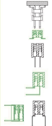
PH200-23SXXXXXXX2
